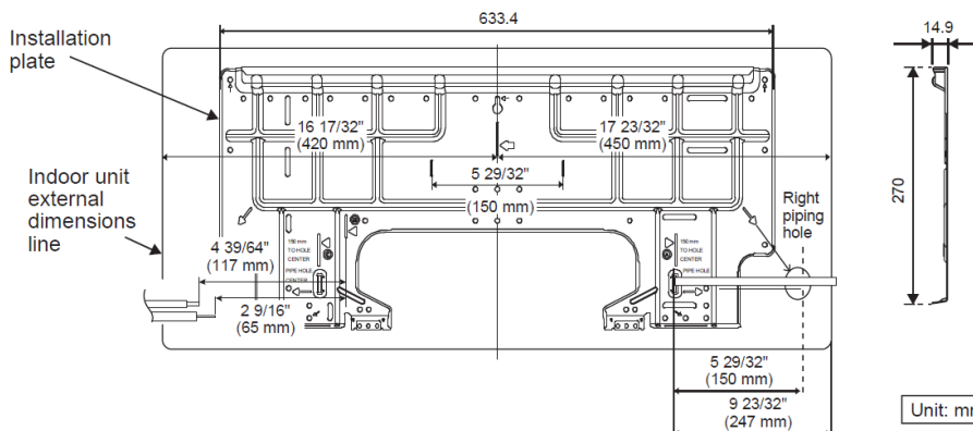
Relative position between the indoor unit and the installation plate &lt;Front View&gt;
